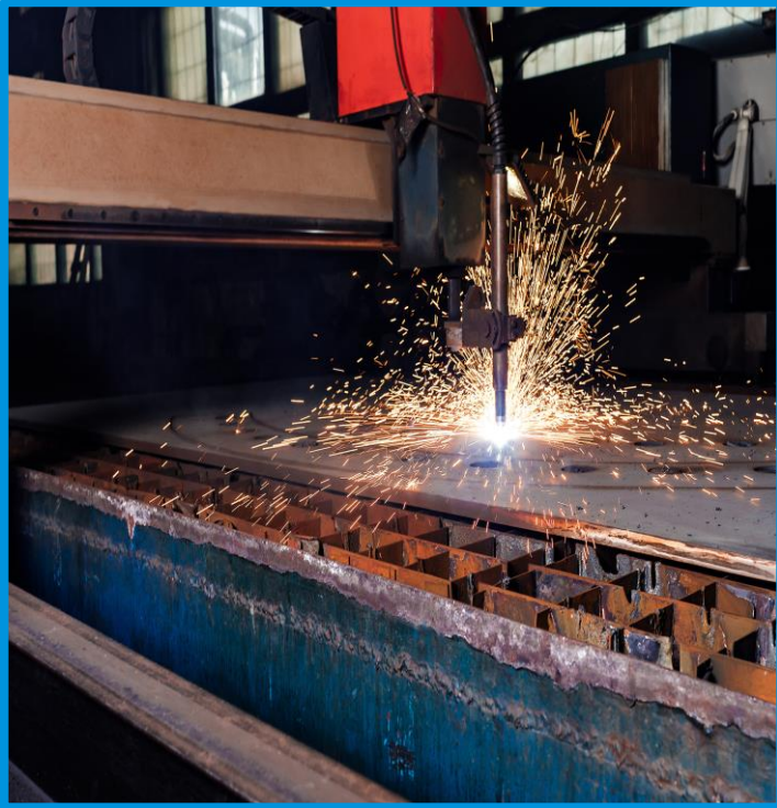
CNC PLASMA MACHINE FOR BASEPLATE AND STAINLESS STEEL CUTTING
